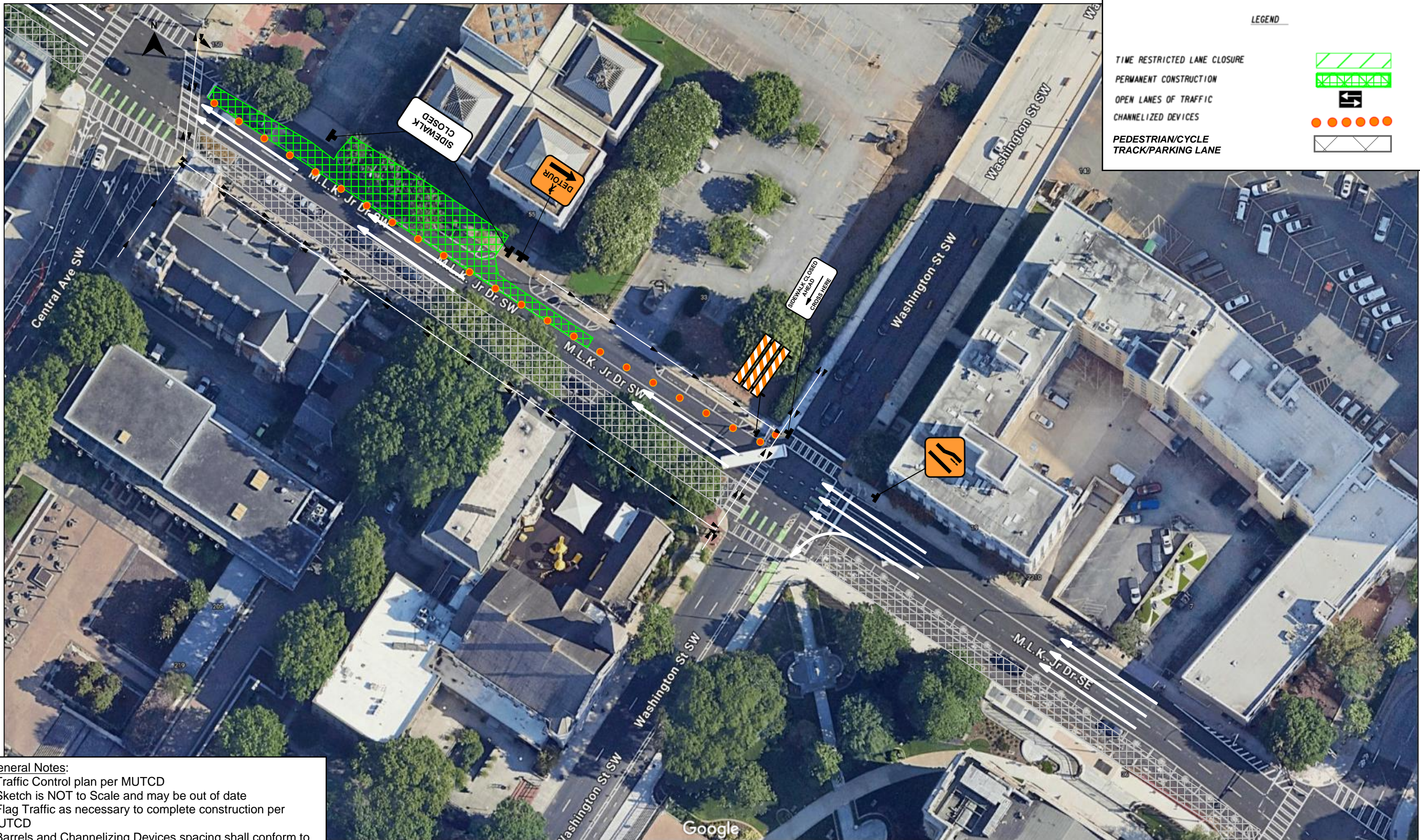
Typical Application - Permanent Bus Lane Closure at Station Locations
