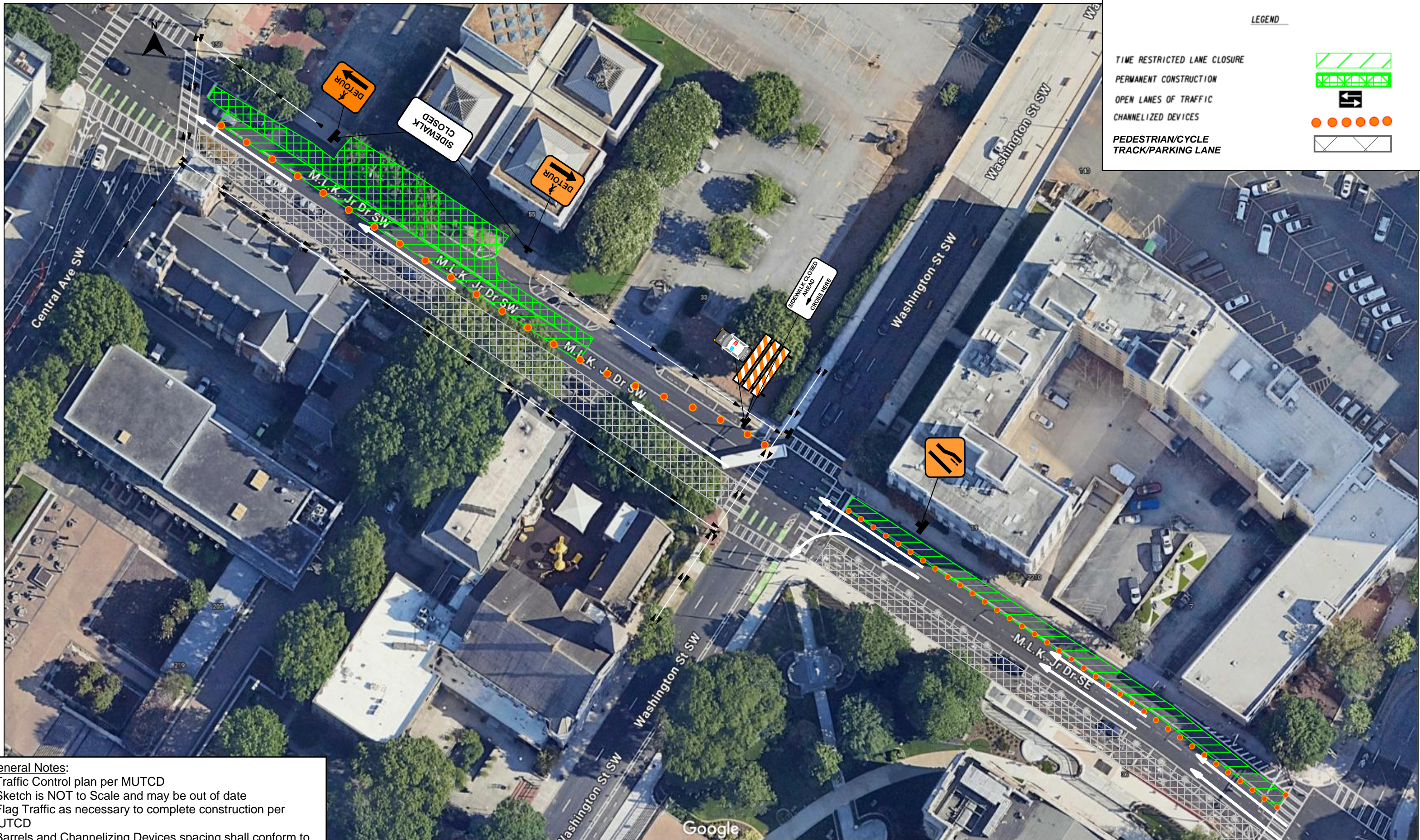
Typical Application - Time Restricted Closure for Major Operations at Station Locations
